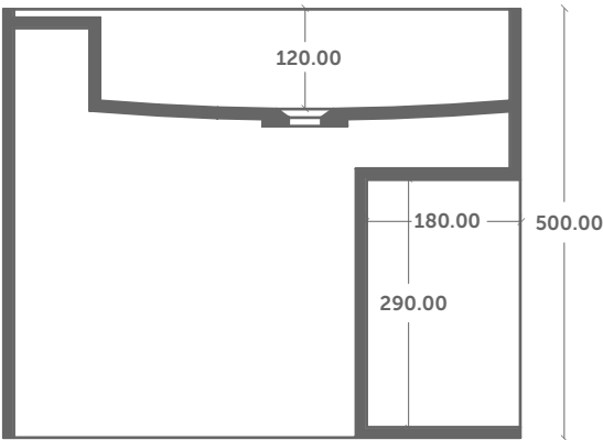
Side Cross Section
