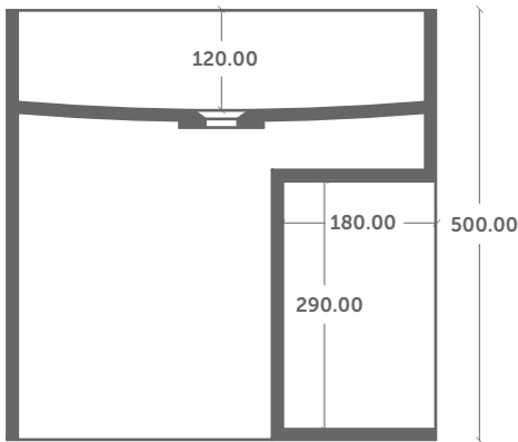
Front Cross Section
