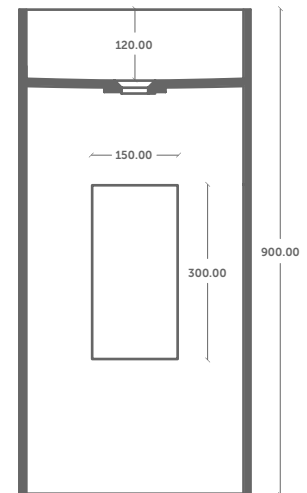
Front Cross Section
